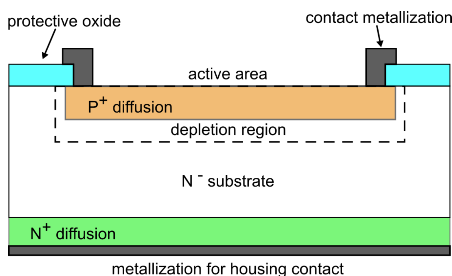
Structure of silicon PIN diode.
