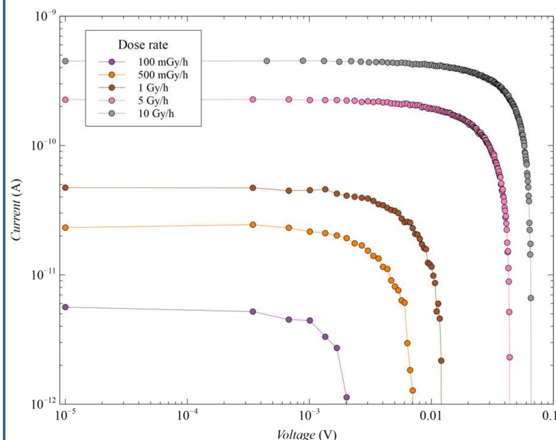
PIN diode with active area 0.8 mm 2 for different dose rates.
