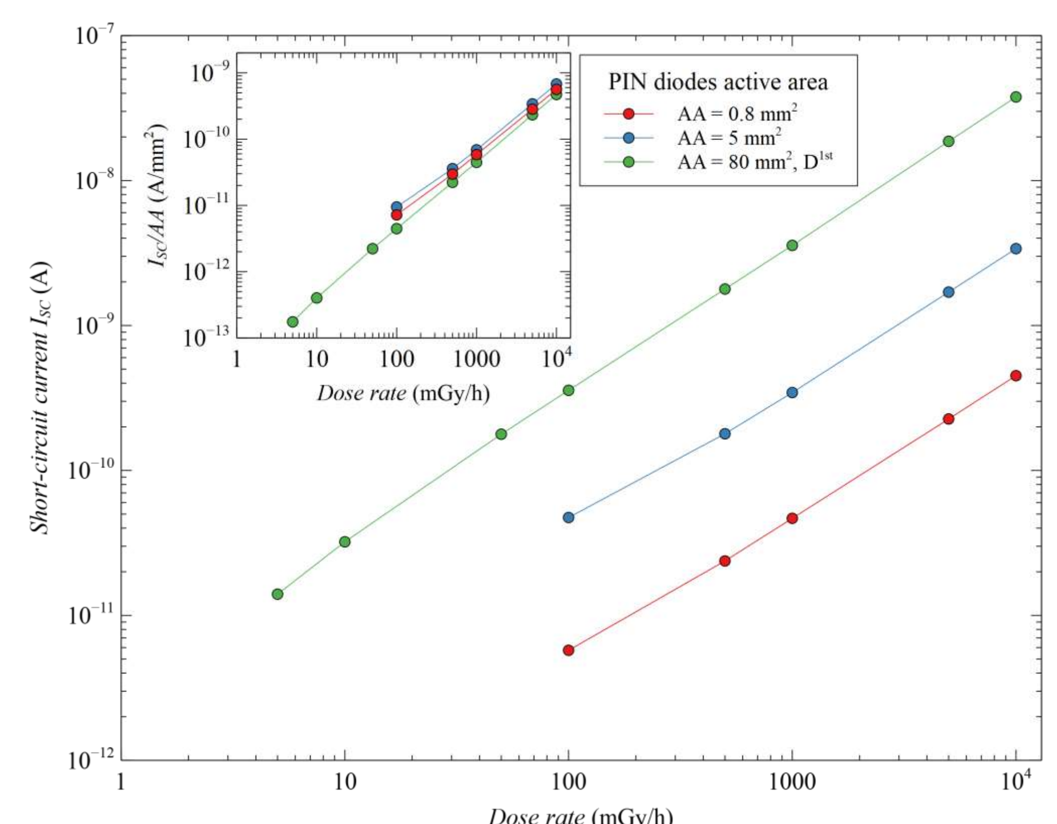
Short-circuit current vales of PIN diodes for different dose rate.
