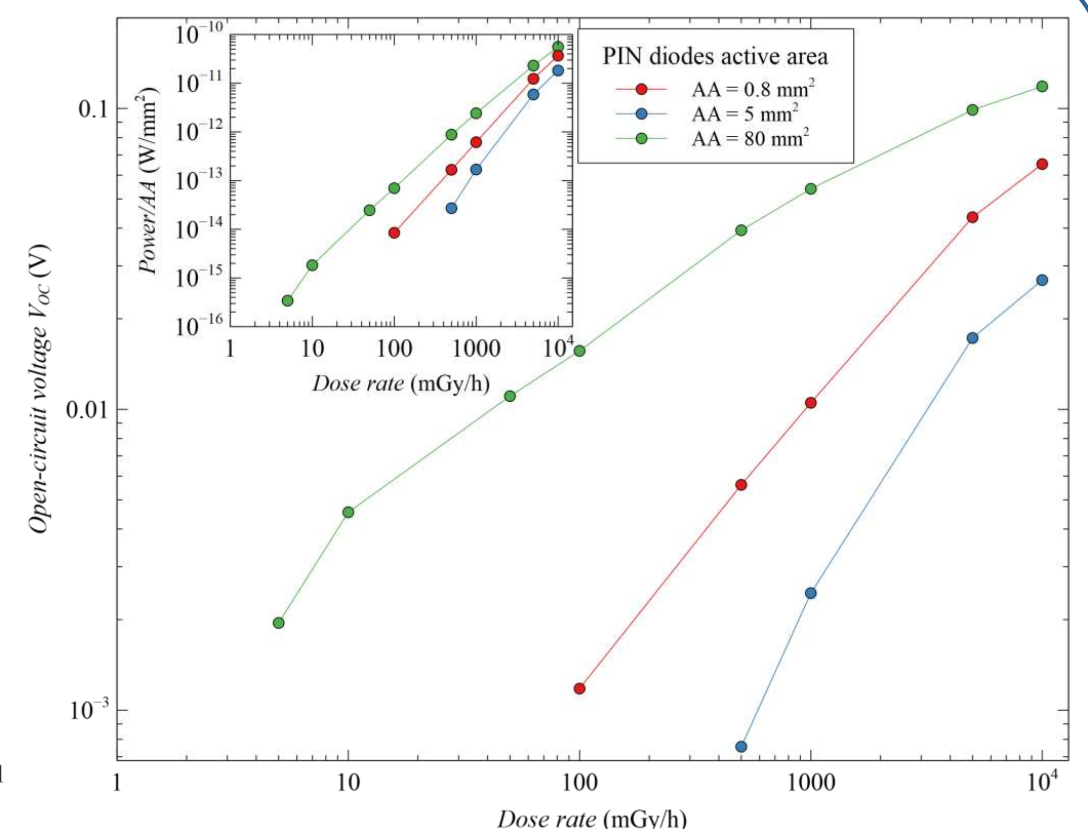
Open-circuit voltage vales of PIN diodes for different dose rate.
