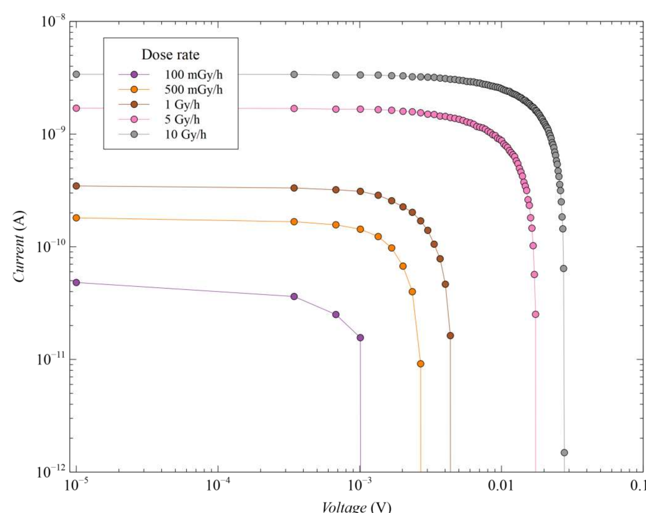
PIN diode with active area 5 mm 2 for different dose rates.
