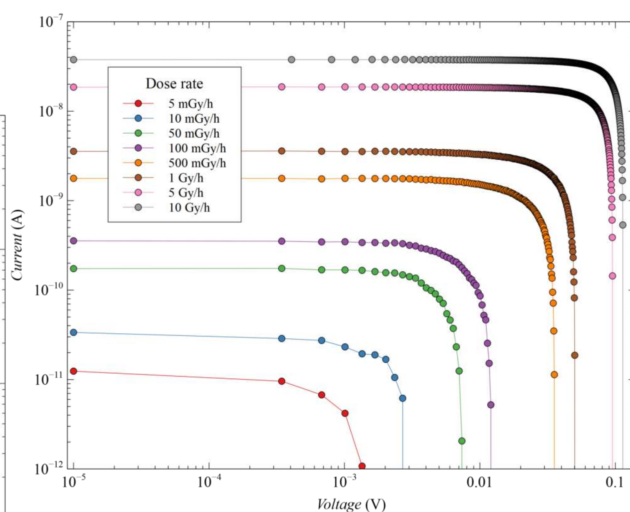
PIN diode with active area 80 mm 2 for different dose rates.
